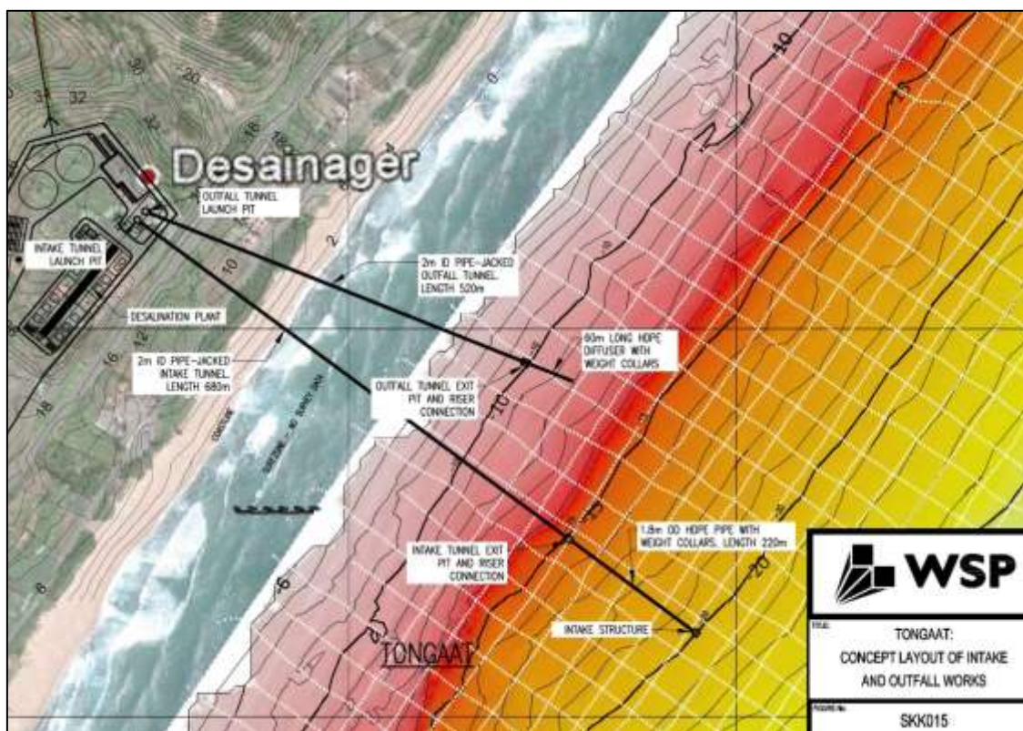
Figure 2.9: Proposed Intake and Outfall Configuration at Tongaat
