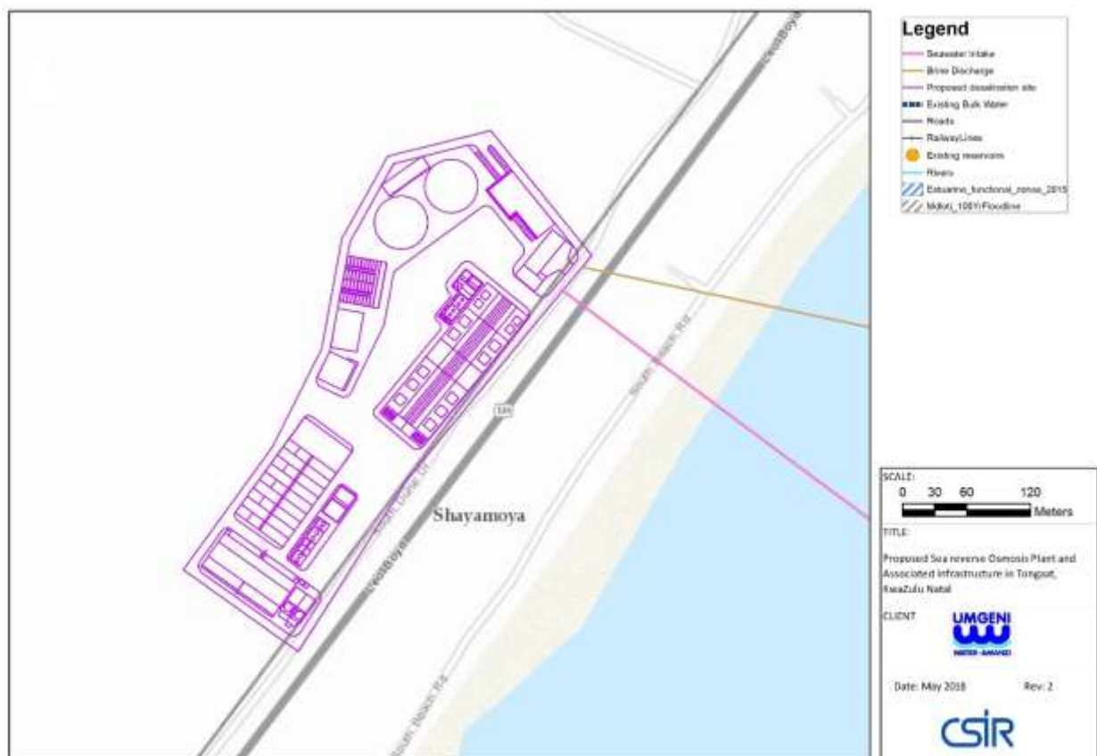
Figure 2-11a: Location of the proposed Tongaat Desalination Plant
