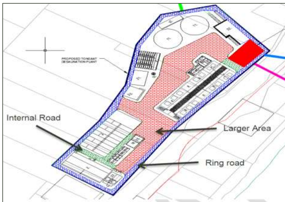
Figure 2-24: Proposed Internal Roads for the Tongaat Desalination Plant
